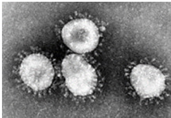
Figure 1: Electron micrograph of a coronavirus
